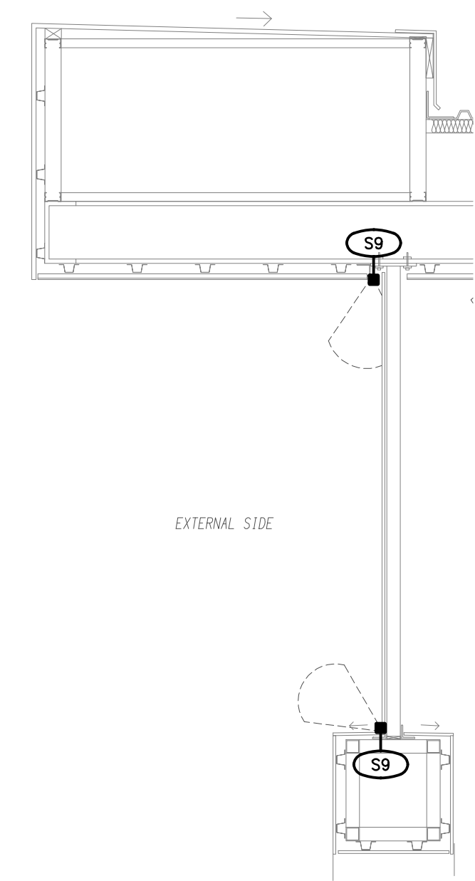
DETAIL A FACADE / ROOF STRIP LIGHT S9 SECTION SCALE 1:20
